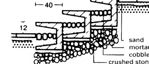
24 Karlsruhe garden stones arranged as concrete steps
